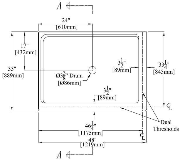
PLAN 48" x 35" [1219mm x 889mm] Corner Shower Pan w/ Dual 6" [152mm] Thresholds Left Hand Version (SP4835L) Shown CENTER DRAIN
